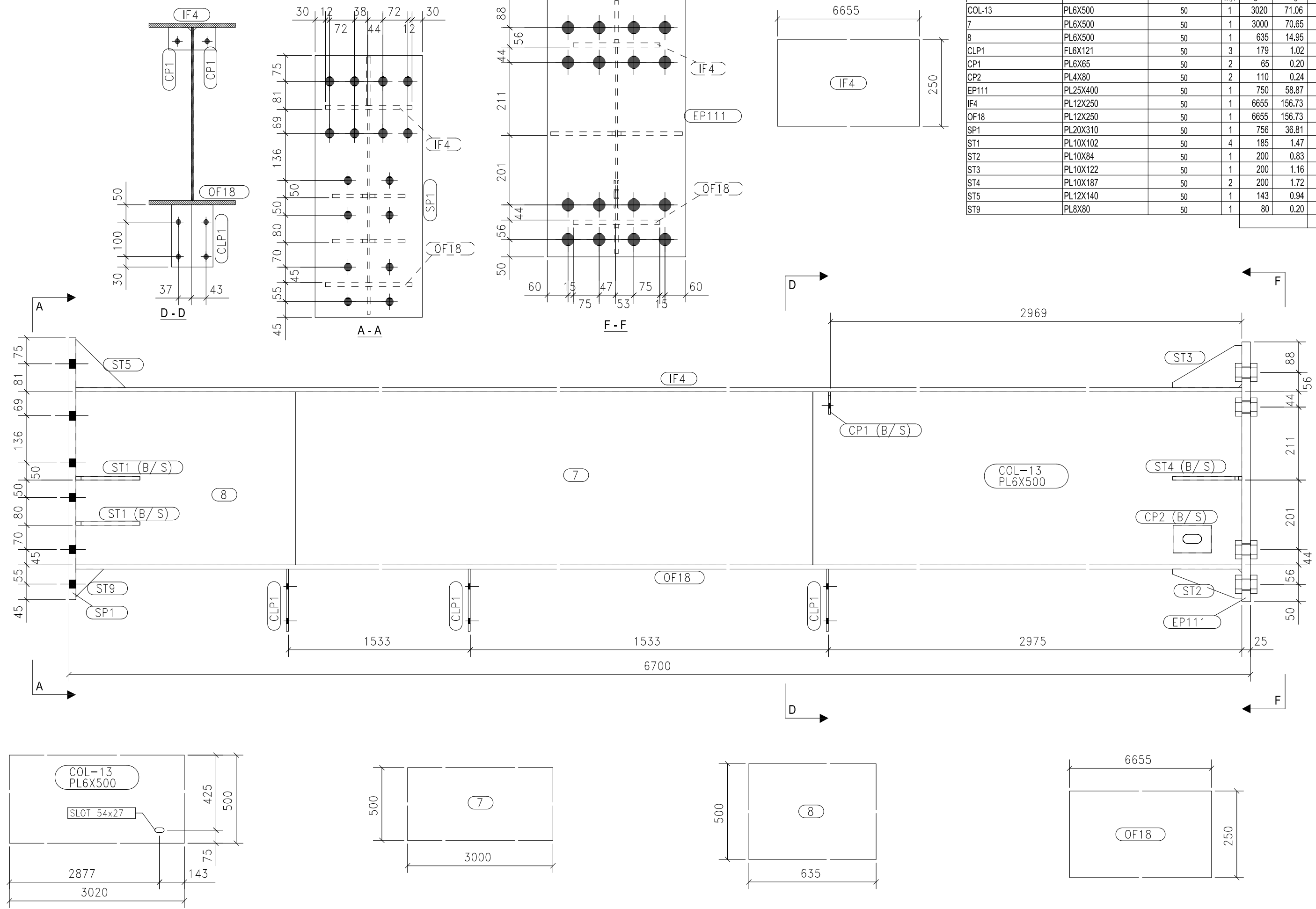
MATERIAL LIST FOR ONE ASSEMBLY MK'D COL-13 2 NO. Required
